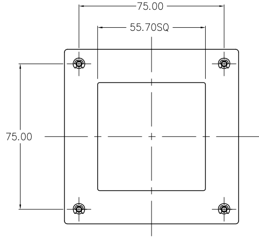
HEATSINK BOTTOM-VIEW
